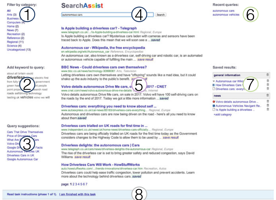
Fig. 7.4 Screenshot SearchAssist: input and control features (first dimension) in ①–④; informational features (second dimension) in ⑤ and personalizable features (third dimension) in ⑥–⑧
